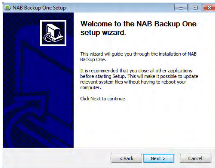
Figure 1: Setup Window
